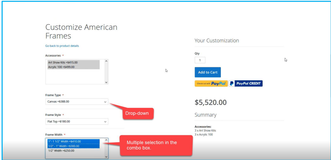
Figure: Multiple Selections option in Combo box.
