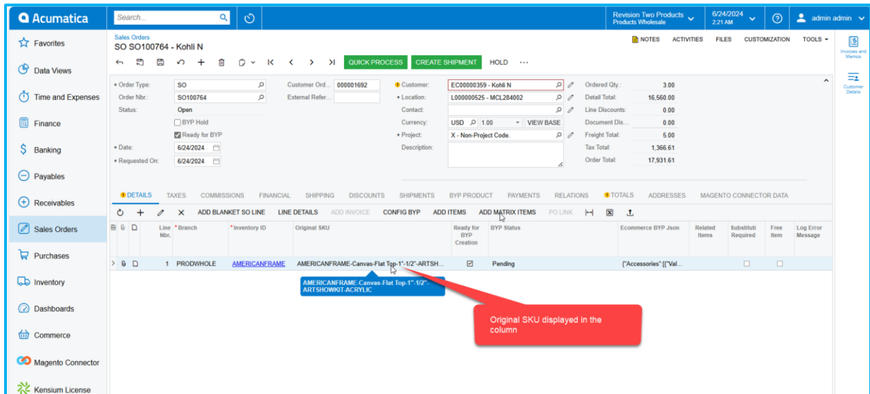
Figure: New Field Original SKU in Sales Order screen
